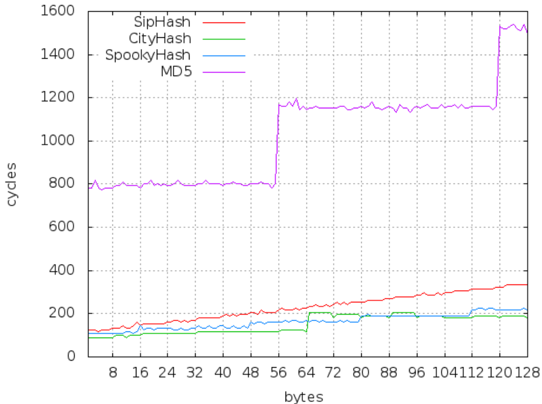
Fig. 6.3. Performance of SipHash-2-4 compared to non-cryptographic hash functions CityHash and SpookyHash and to MD5 on “latour” (Intel Core 2 Quad Q6600), for messages of 1, 2, ..., 128 bytes. Curves on the right, from top to bottom, are MD5, SipHash, SpookyHash, and CityHash.
