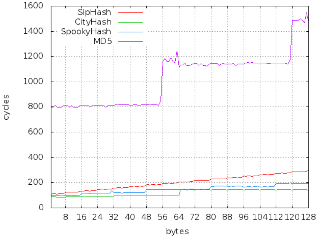
Fig. 6.2. Performance of SipHash-2-4 compared to non-cryptographic hash functions CityHash and SpookyHash and to MD5 on “ishmael” (AMD Athlon II), for messages of 1, 2, . . . , 128 bytes. Curves on the right, from top to bottom, are MD5, SipHash, SpookyHash, and CityHash.
