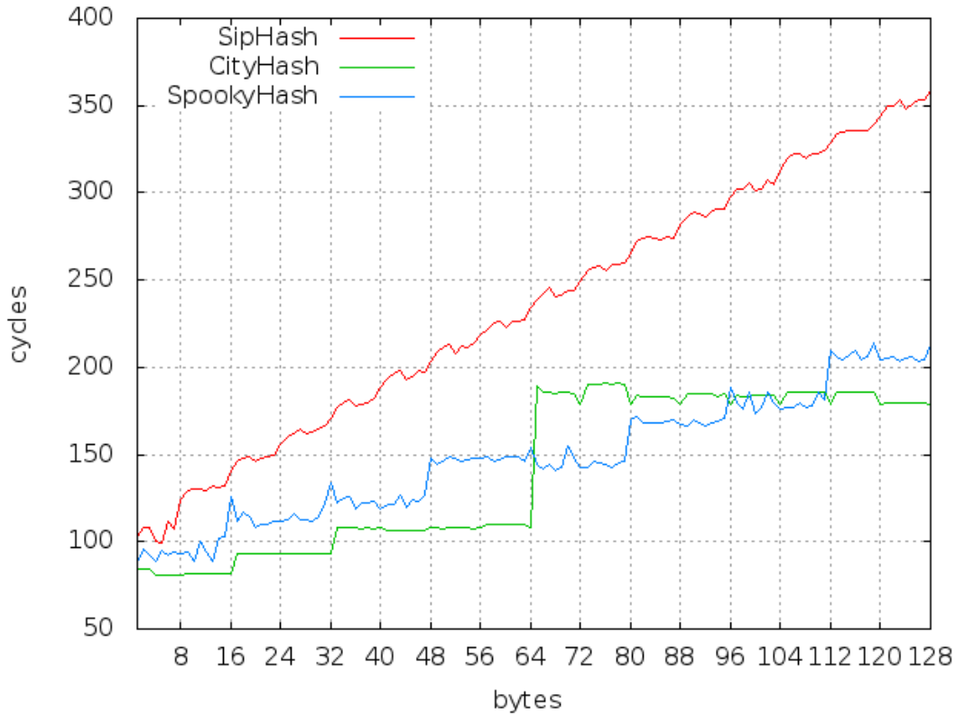
Fig. 6.4. Performance of SipHash-2-4 compared to non-cryptographic hash functions CityHash and SpookyHash on “bulldozer” (AMD FX-8150), for messages of 1, 2, . . . , 128 bytes. Curves on the right, from top to bottom, are SipHash, SpookyHash, and CityHash.
